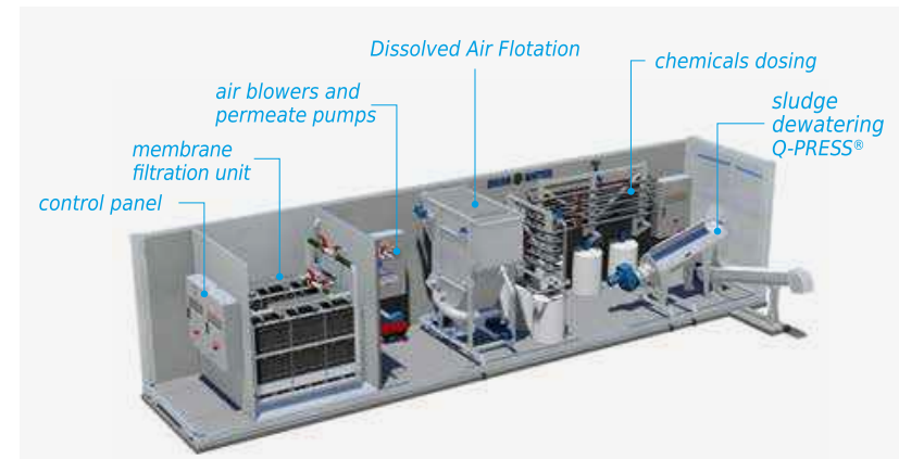
Package plants for industrial wastewater treatment.
