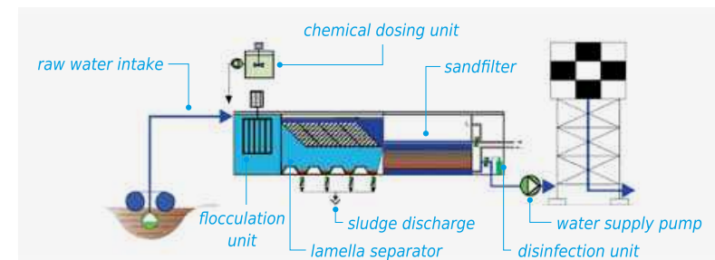
Optimized process scheme to achieve high quality drinking water.
